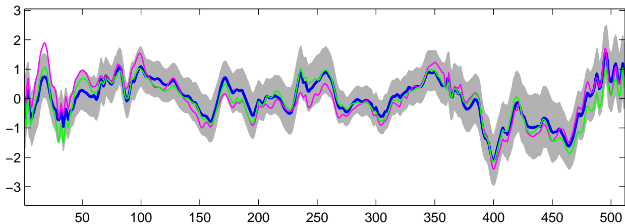
Estimated U_{28}(t) using R-WFMM: Normal data, run 9
