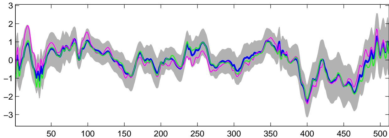
Estimated U_{28}(t) using G-WFMM: Normal data, run 9
