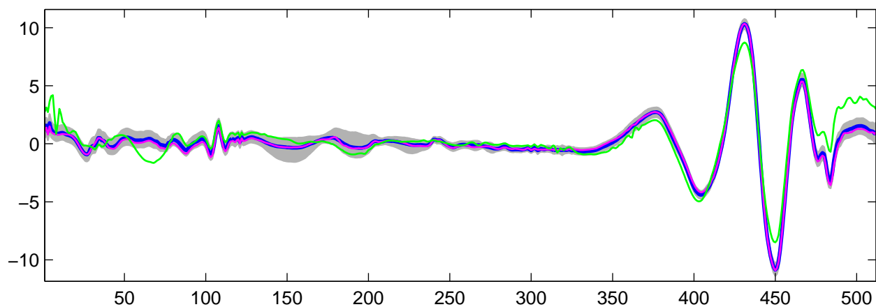
Estimated U_{28}(t) using R-WFMM: t_1 data, run 9
