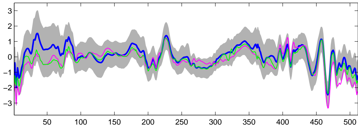
Estimated U_{28}(t) using G-WFMM: t_2 data, run 9
