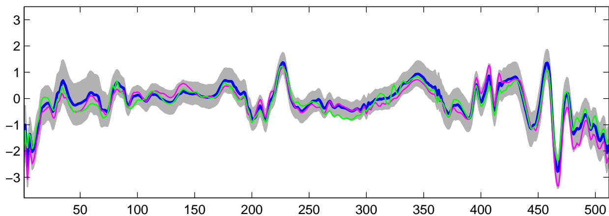
Estimated U_{28}(t) using R-WFMM: t_2 data, run 9
