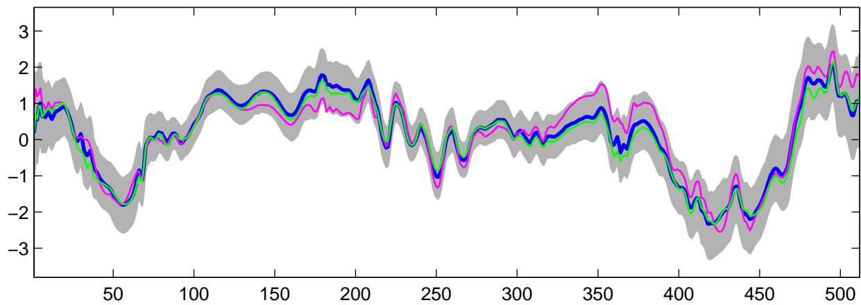
Estimated U_{28}(t) using G-WFMM: t_3 data, run 9
