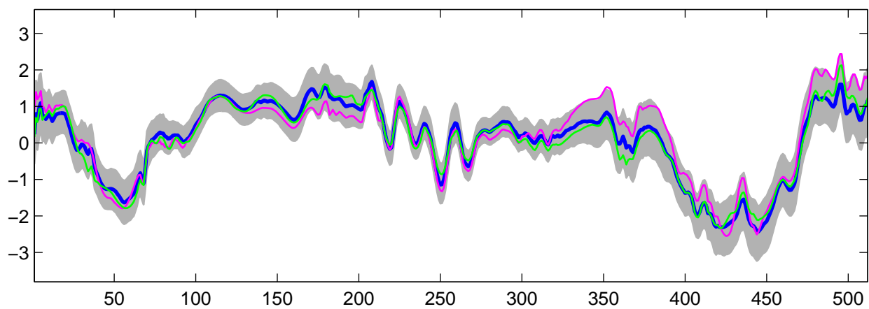
Estimated U_{28}(t) using R-WFMM: t_3 data, run 9
