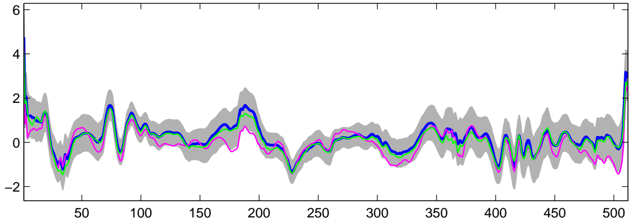
Estimated U_{29}(t) using G-WFMM: DE data, run 9
