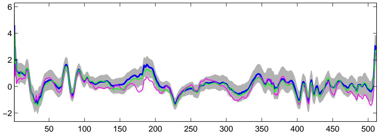
Estimated U_{29}(t) using R-WFMM: DE data, run 9
