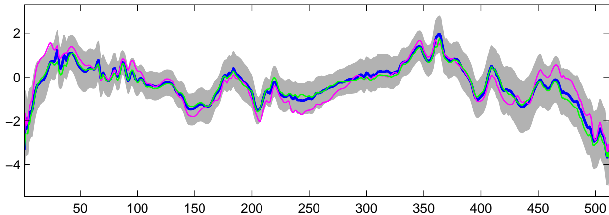
Estimated U_{29}(t) using G-WFMM: Normal data, run 9
