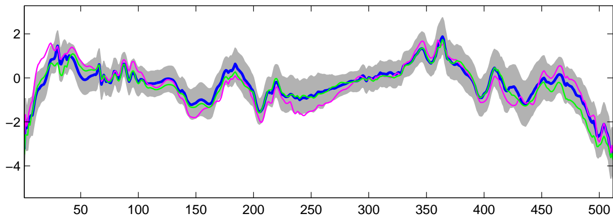
Estimated U_{29}(t) using R-WFMM: Normal data, run 9
