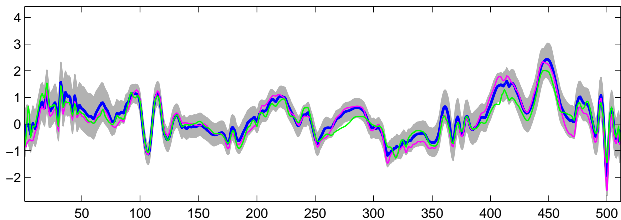
Estimated U_{29}(t) using R-WFMM: t_2 data, run 9
