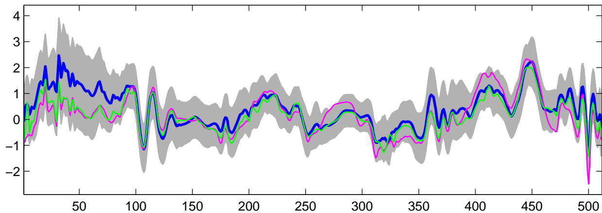
Estimated U_{29}(t) using G-WFMM: t_2 data, run 9
