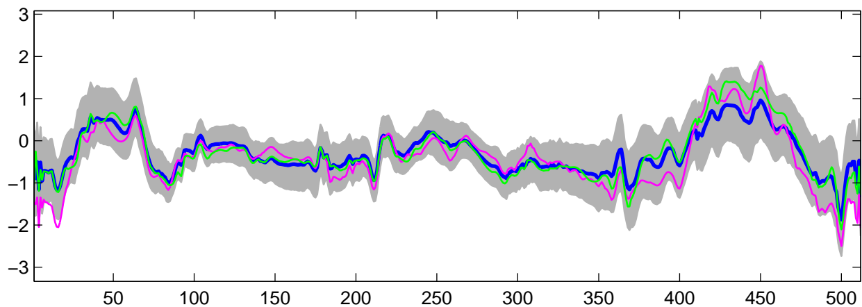
Estimated U_2(t) using R-WFMM: DE data, run 9
