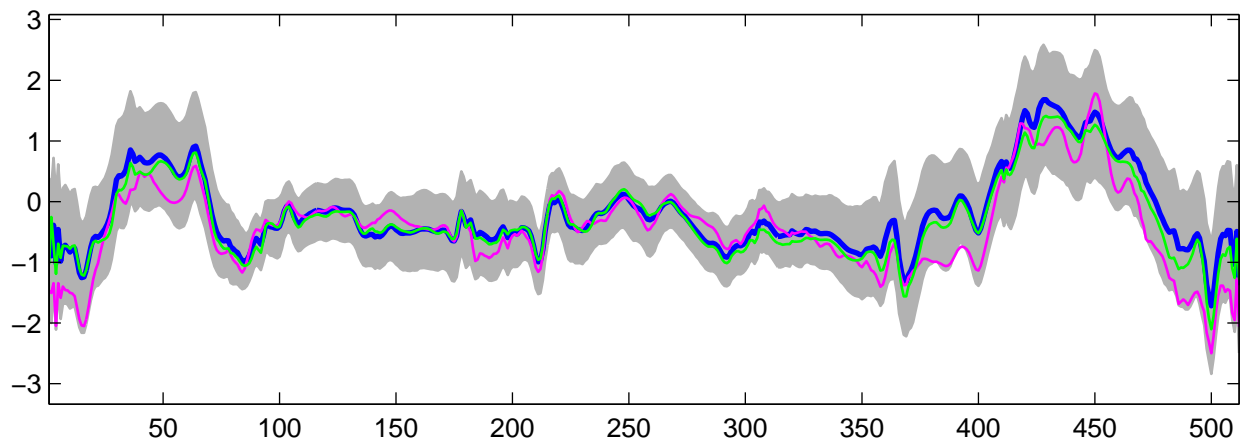
Estimated U_2(t) using G-WFMM: DE data, run 9
