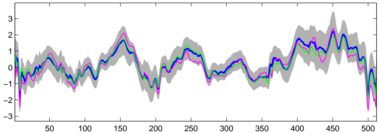
Estimated U_2(t) using R-WFMM: Normal data, run 9
