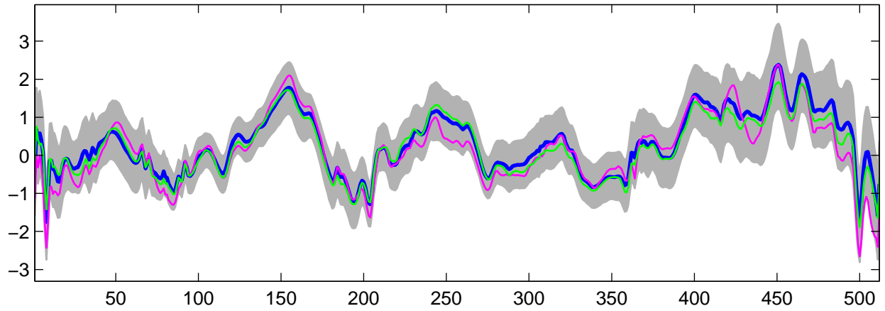
Estimated U_2(t) using G-WFMM: Normal data, run 9
