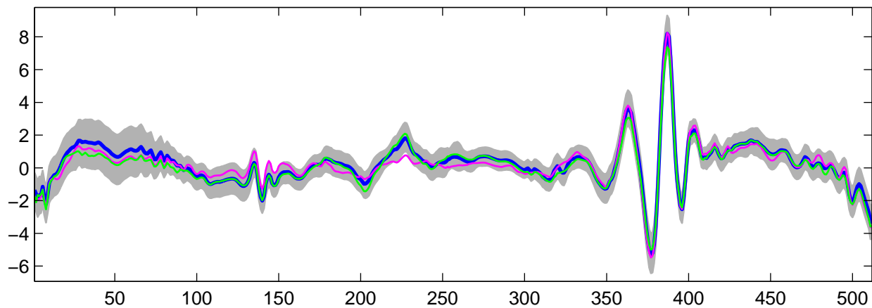
Estimated U_2(t) using G-WFMM: t_2 data, run 9
