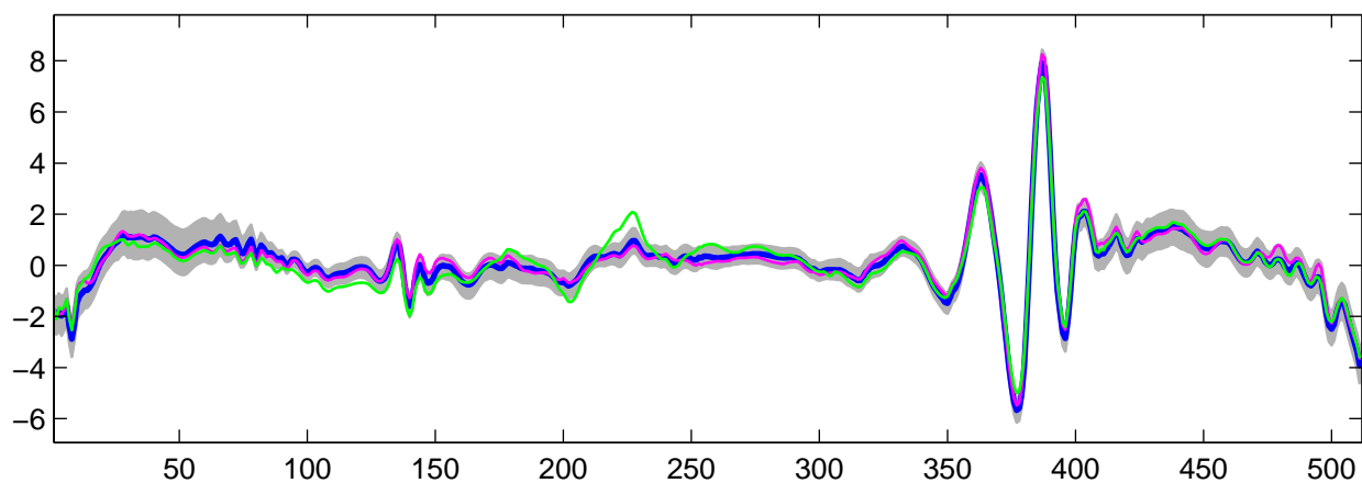
Estimated U_2(t) using R-WFMM: t_2 data, run 9
