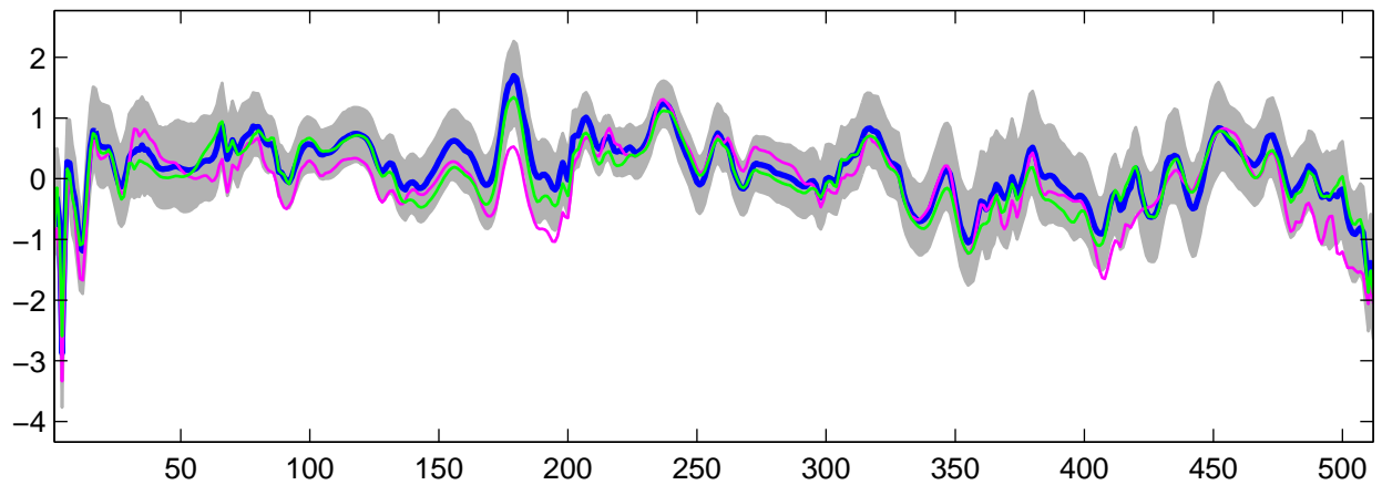
Estimated U_{30}(t) using R-WFMM: DE data, run 9
