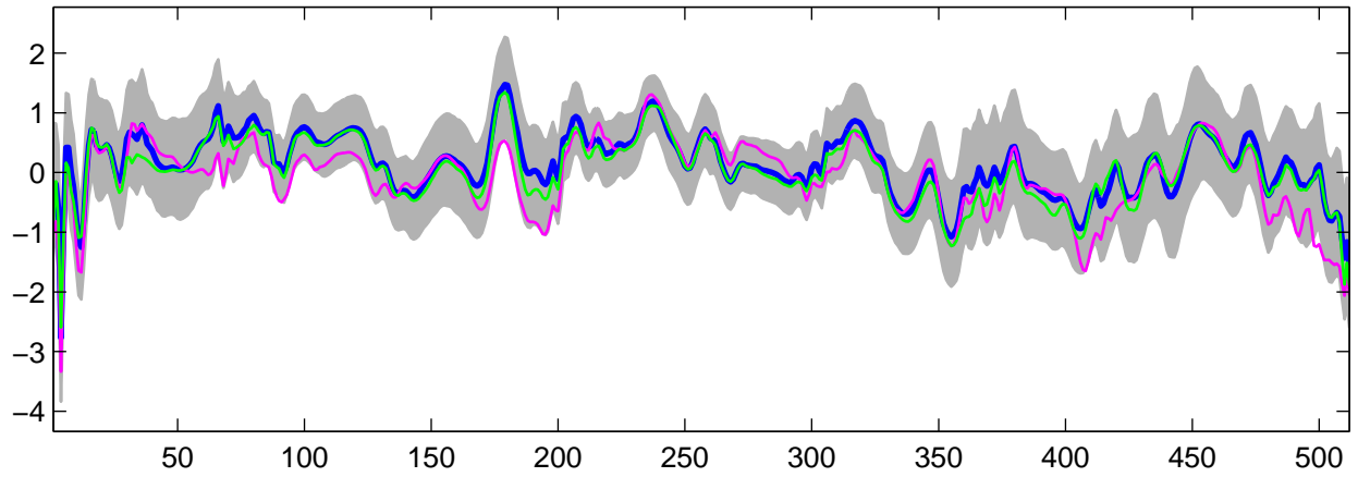
Estimated U_{30}(t) using G-WFMM: DE data, run 9
