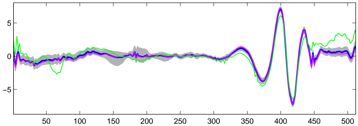
Estimated U_{30}(t) using R-WFMM: t_1 data, run 9
