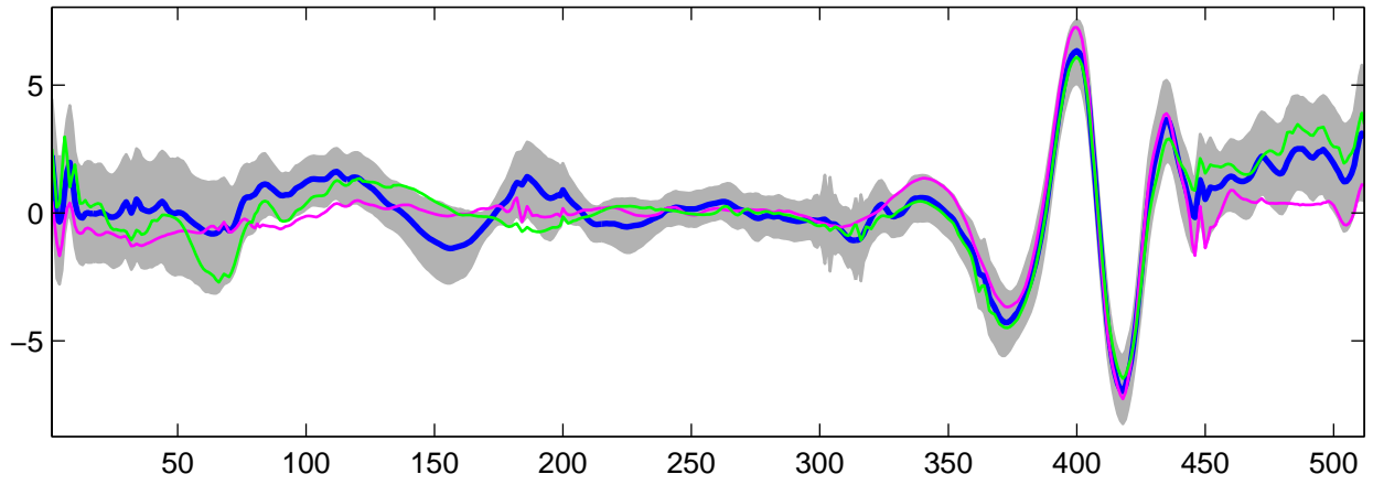
Estimated U_{30}(t) using G-WFMM: t_1 data, run 9
