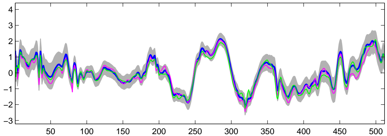
Estimated U_{30}(t) using R-WFMM: t_2 data, run 9
