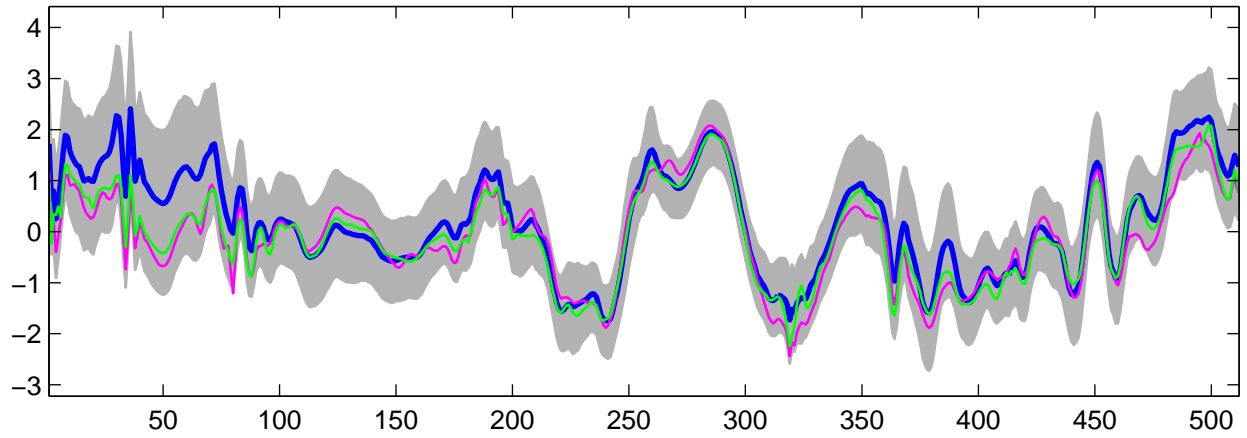
Estimated U_{30}(t) using G-WFMM: t_2 data, run 9
