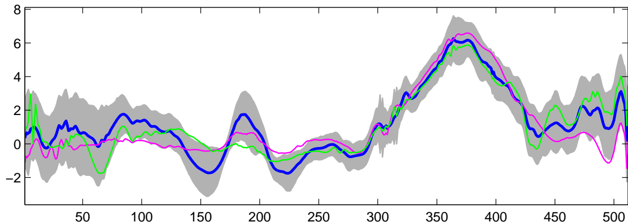
Estimated U_{31}(t) using G-WFMM: t_1 data, run 9
