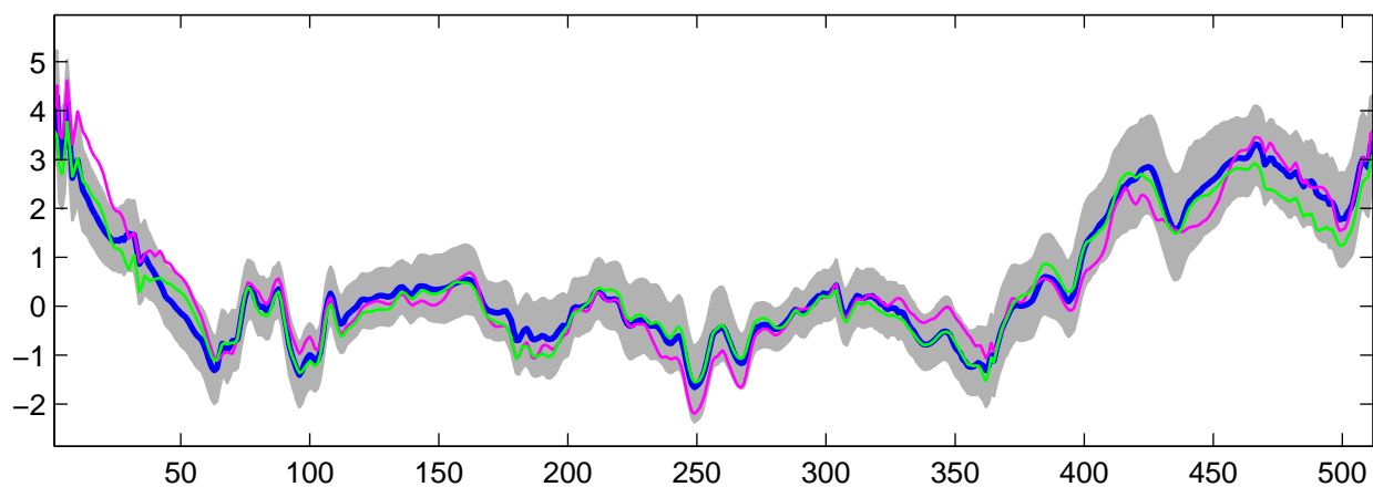
Estimated U_{32}(t) using R-WFMM: Normal data, run 9
