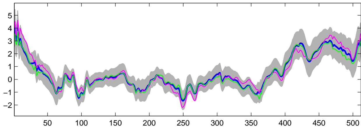
Estimated U_{32}(t) using G-WFMM: Normal data, run 9
