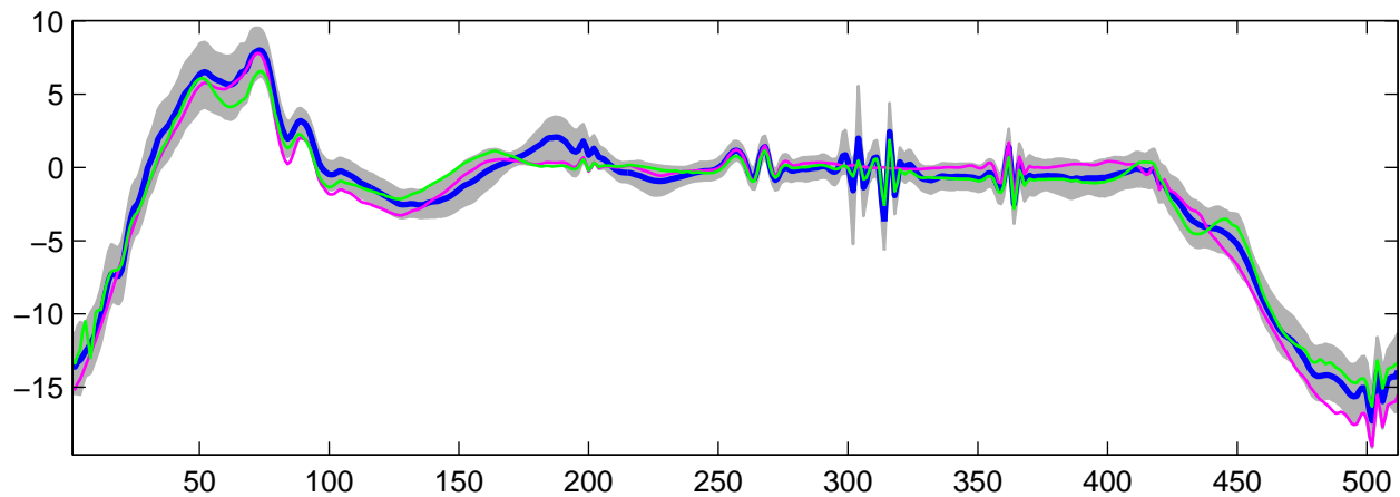
Estimated U_{32}(t) using G-WFMM: t_1 data, run 9
