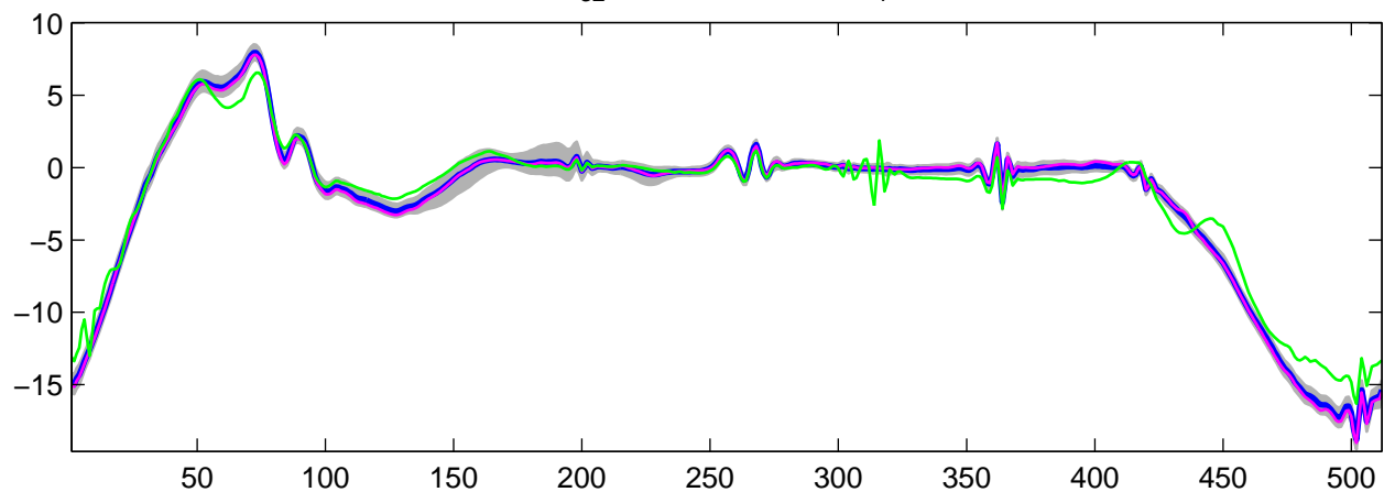
Estimated U_{32}(t) using R-WFMM: t_1 data, run 9
