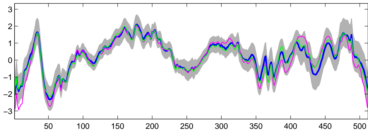
Estimated U_3(t) using R-WFMM: DE data, run 9
