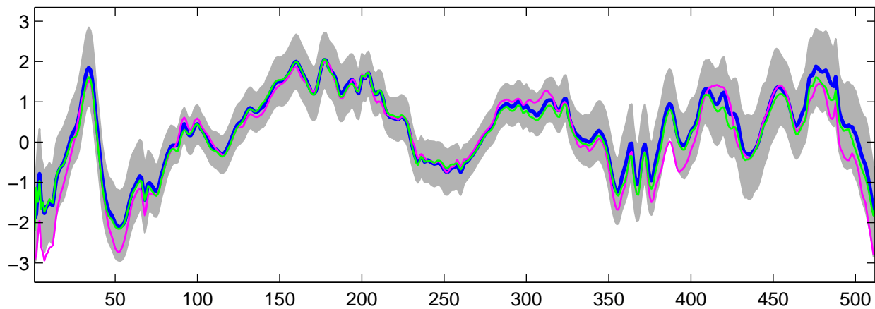
Estimated U_3(t) using G-WFMM: DE data, run 9
