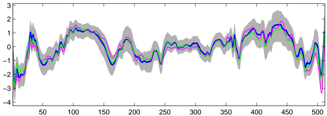
Estimated U_3(t) using R-WFMM: Normal data, run 9
