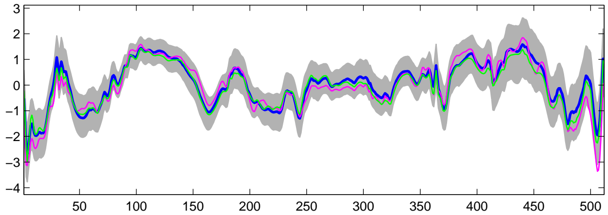
Estimated U_3(t) using G-WFMM: Normal data, run 9
