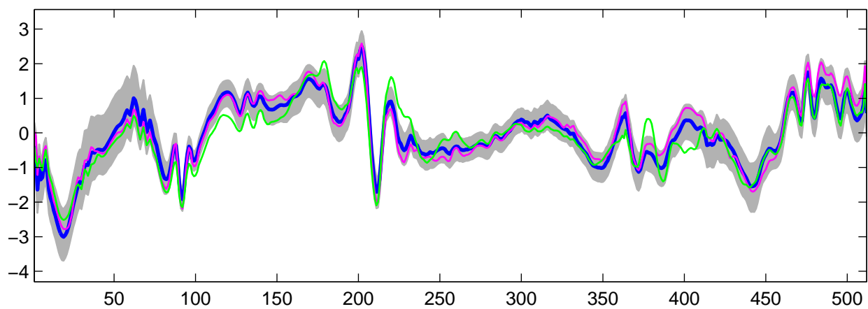
Estimated U_3(t) using R-WFMM: t_2 data, run 9
