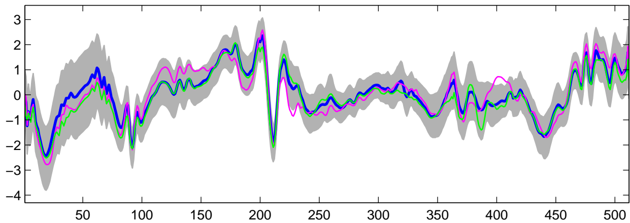
Estimated U_3(t) using G-WFMM: t_2 data, run 9
