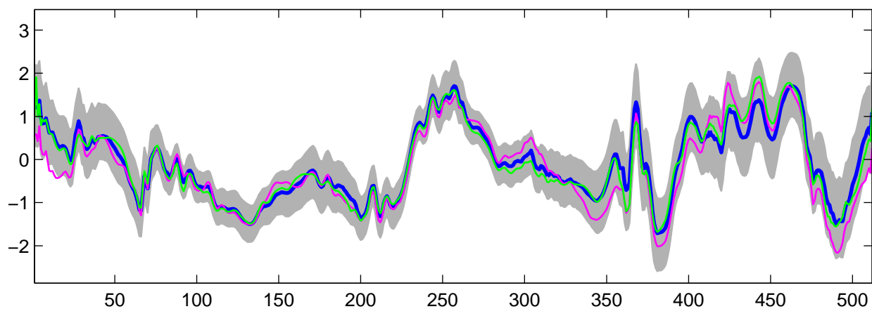
Estimated U_4(t) using R-WFMM: DE data, run 9
