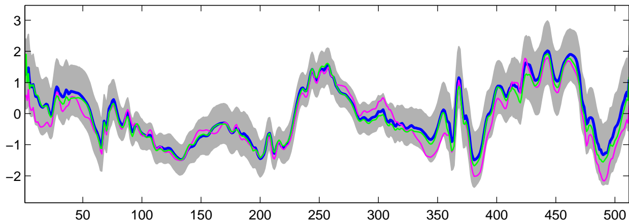
Estimated U_4(t) using G-WFMM: DE data, run 9
