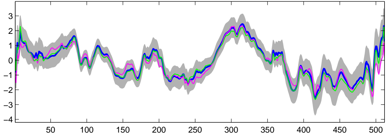
Estimated U_4(t) using G-WFMM: Normal data, run 9
