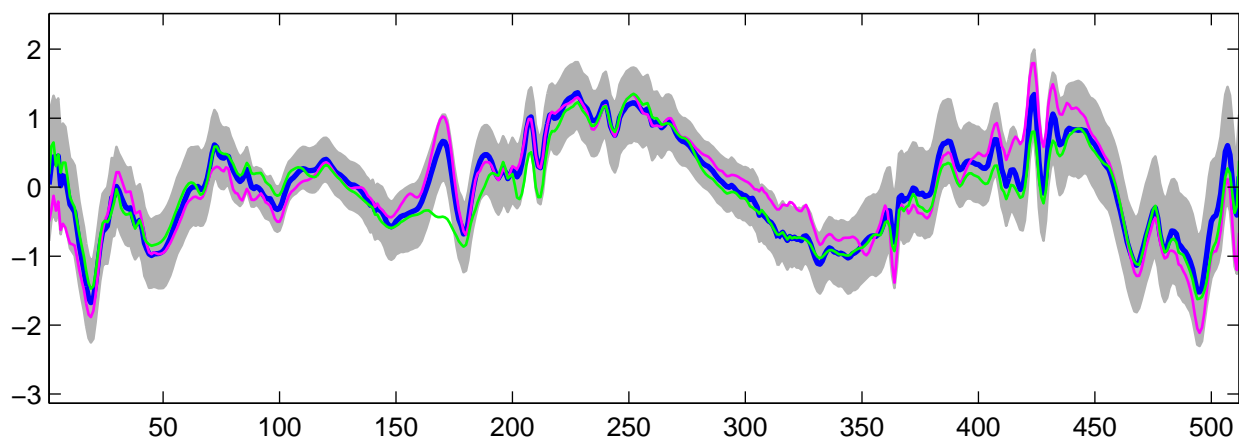
Estimated U_4(t) using R-WFMM: t_3 data, run 9
