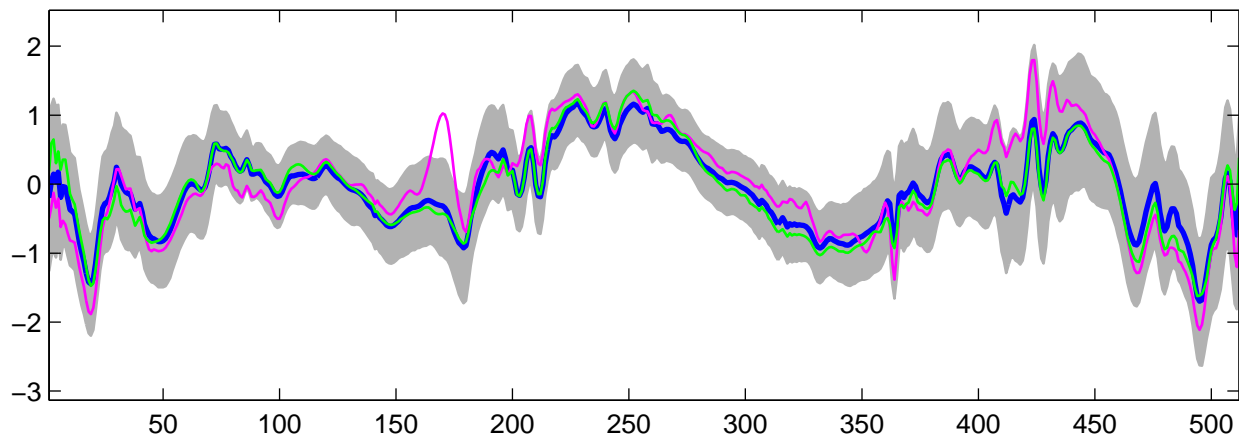
Estimated U_4(t) using G-WFMM: t_3 data, run 9
