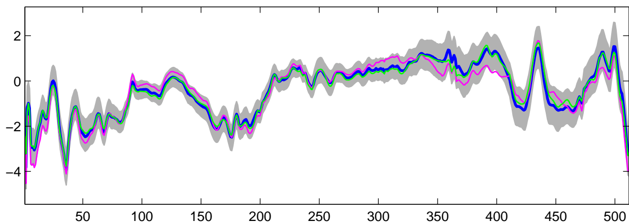
Estimated U_5(t) using R-WFMM: DE data, run 9
