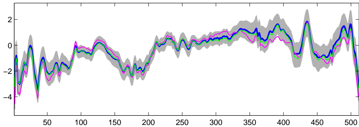
Estimated U_5(t) using G-WFMM: DE data, run 9
