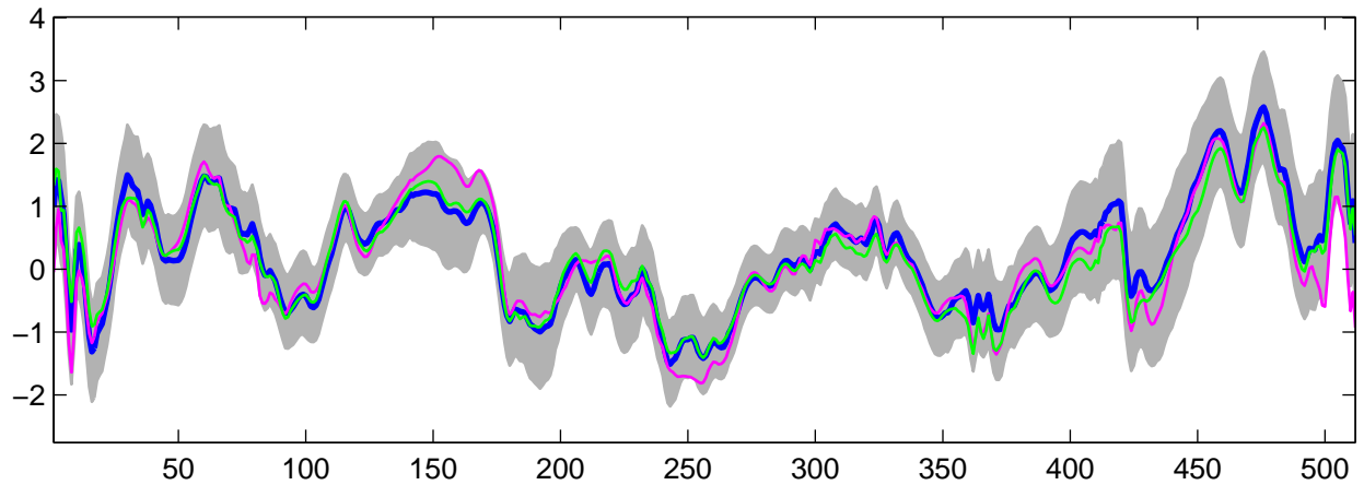
Estimated U_5(t) using R-WFMM: Normal data, run 9
