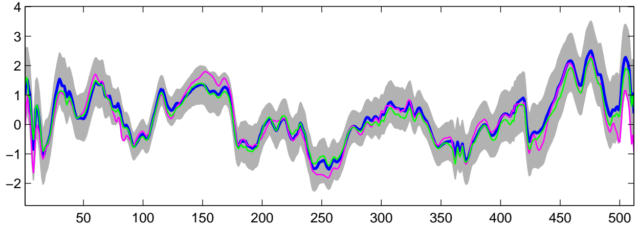
Estimated U_5(t) using G-WFMM: Normal data, run 9
