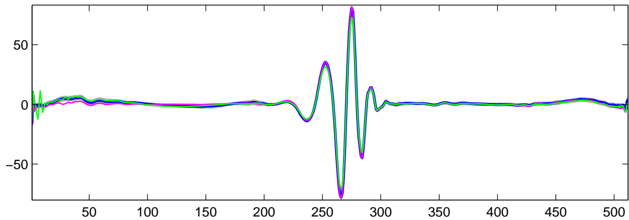
Estimated U_5(t) using G-WFMM: t_1 data, run 9
