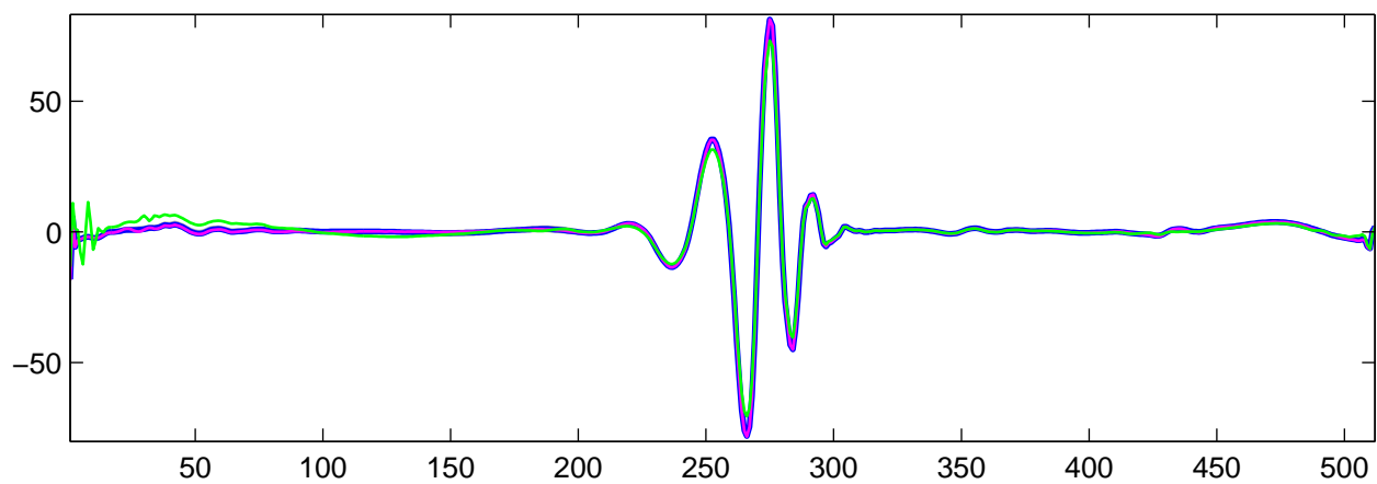
Estimated U_5(t) using R-WFMM: t_1 data, run 9
