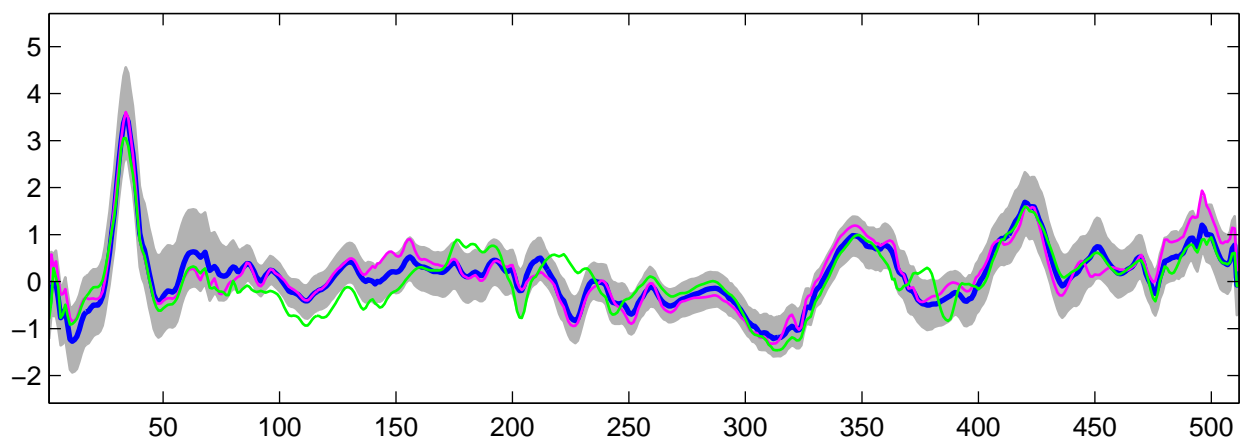
Estimated U_5(t) using R-WFMM: t_2 data, run 9
