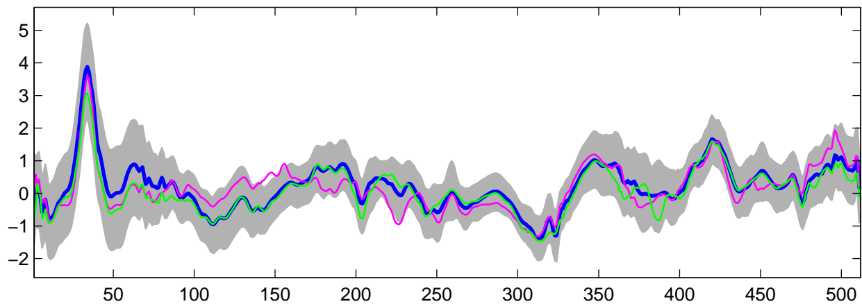
Estimated U_5(t) using G-WFMM: t_2 data, run 9
