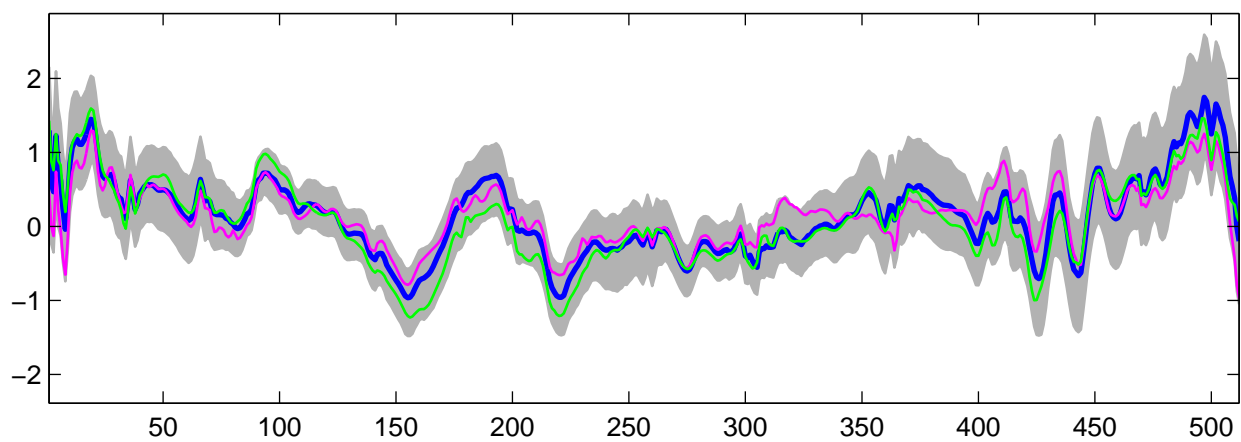
Estimated U_5(t) using R-WFMM: t_3 data, run 9
