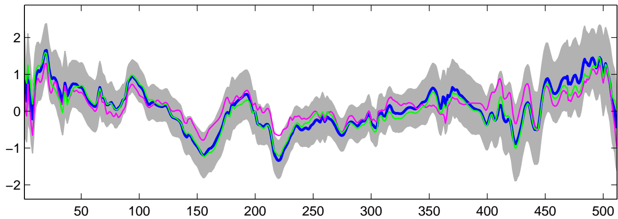
Estimated U_5(t) using G-WFMM: t_3 data, run 9
