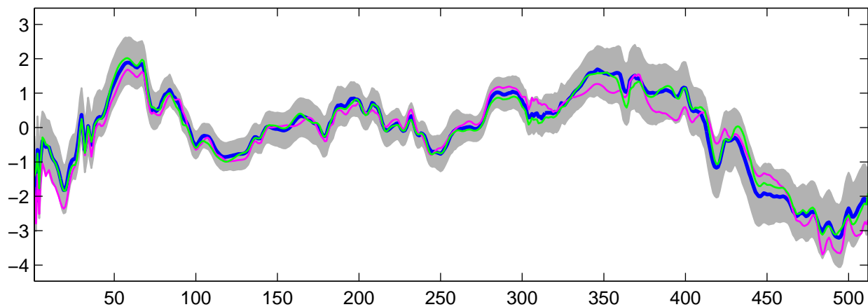
Estimated U_6(t) using R-WFMM: DE data, run 9
