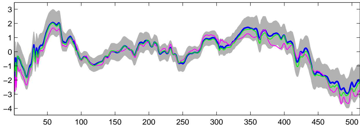
Estimated U_6(t) using G-WFMM: DE data, run 9
