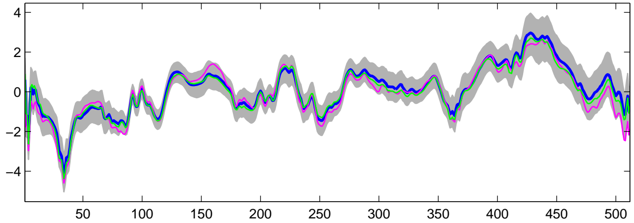
Estimated U_6(t) using G-WFMM: Normal data, run 9
