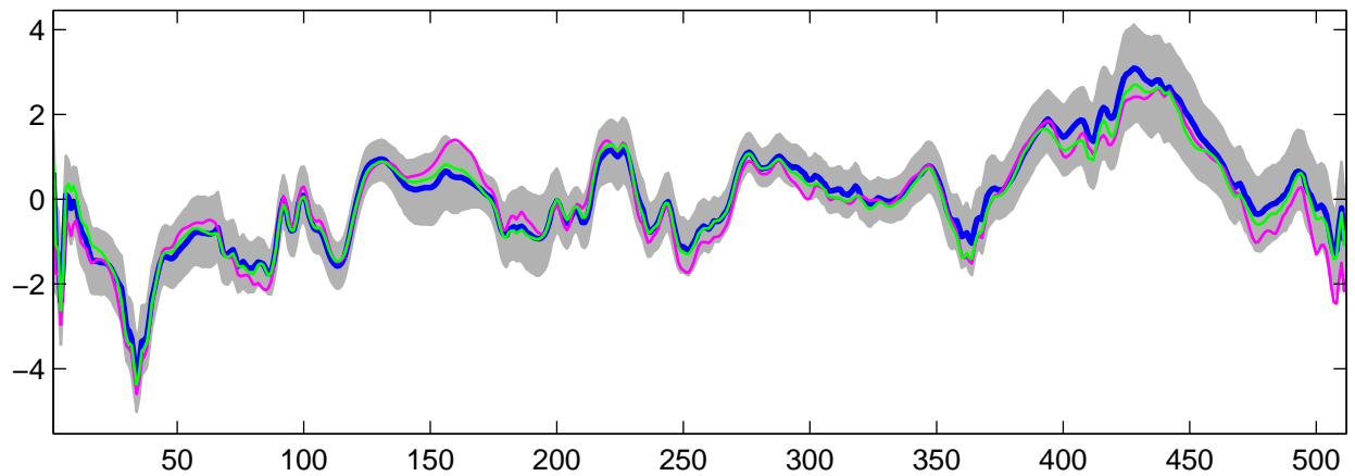
Estimated U_6(t) using R-WFMM: Normal data, run 9
