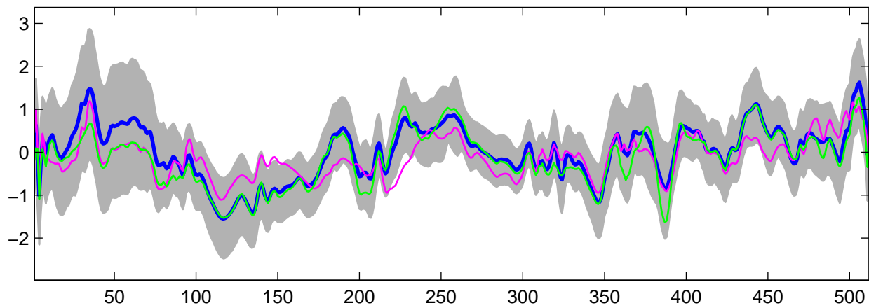
Estimated U_6(t) using G-WFMM: t_2 data, run 9
