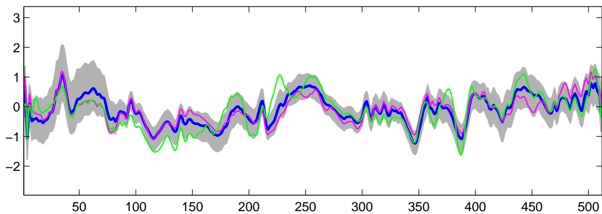
Estimated U_6(t) using R-WFMM: t_2 data, run 9
