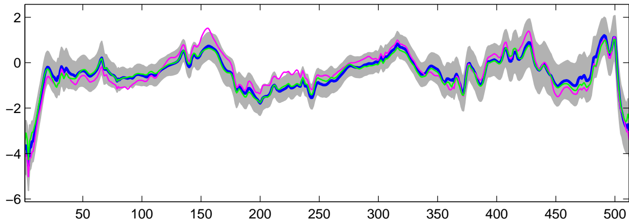
Estimated U_6(t) using G-WFMM: t_3 data, run 9
