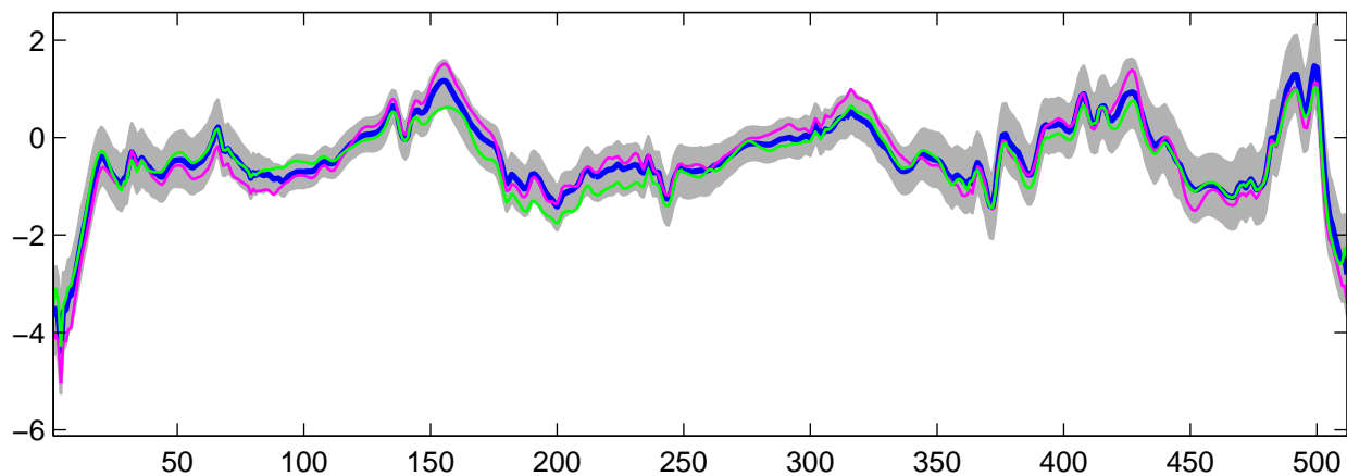
Estimated U_6(t) using R-WFMM: t_3 data, run 9
