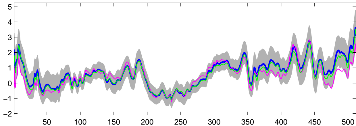
Estimated U_7(t) using G-WFMM: DE data, run 9
