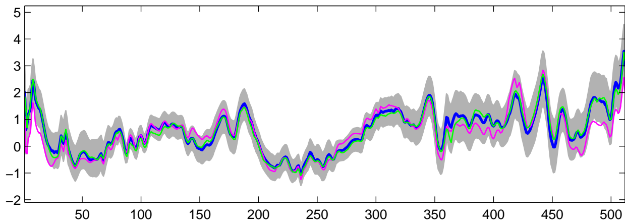
Estimated U_7(t) using R-WFMM: DE data, run 9
