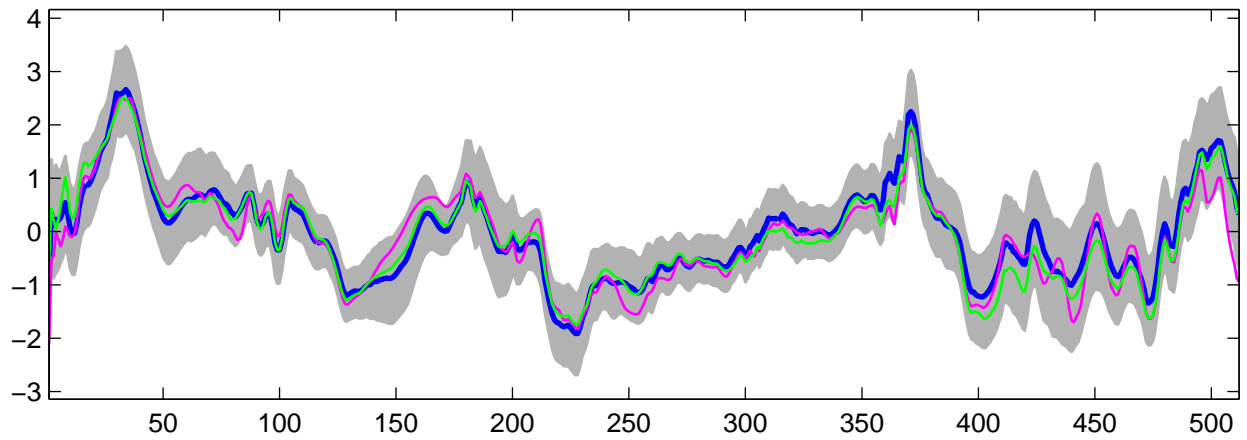
Estimated U_7(t) using R-WFMM: Normal data, run 9
