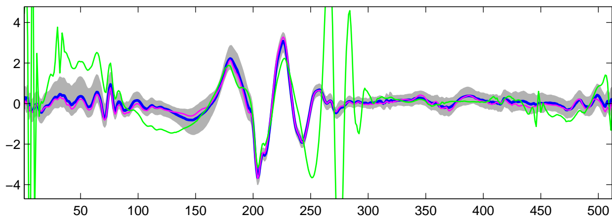
Estimated U_7(t) using R-WFMM: t_1 data, run 9
