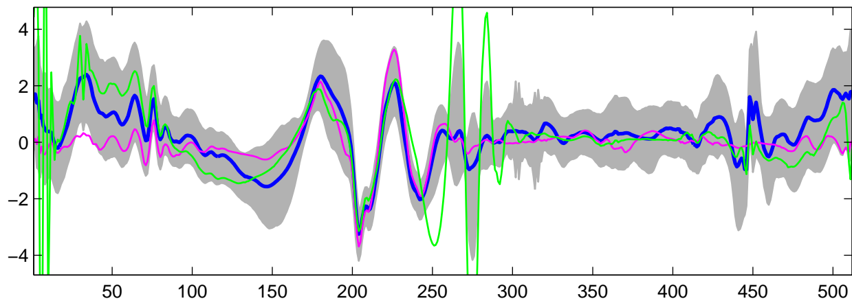
Estimated U_7(t) using G-WFMM: t_1 data, run 9
