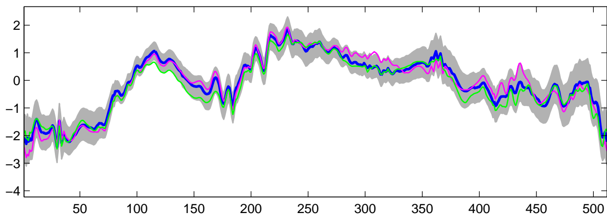
Estimated U_7(t) using R-WFMM: t_3 data, run 9
