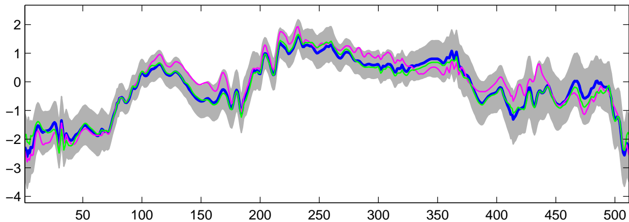
Estimated U_7(t) using G-WFMM: t_3 data, run 9
