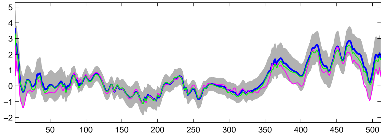
Estimated U_g(t) using G-WFMM: DE data, run 9
