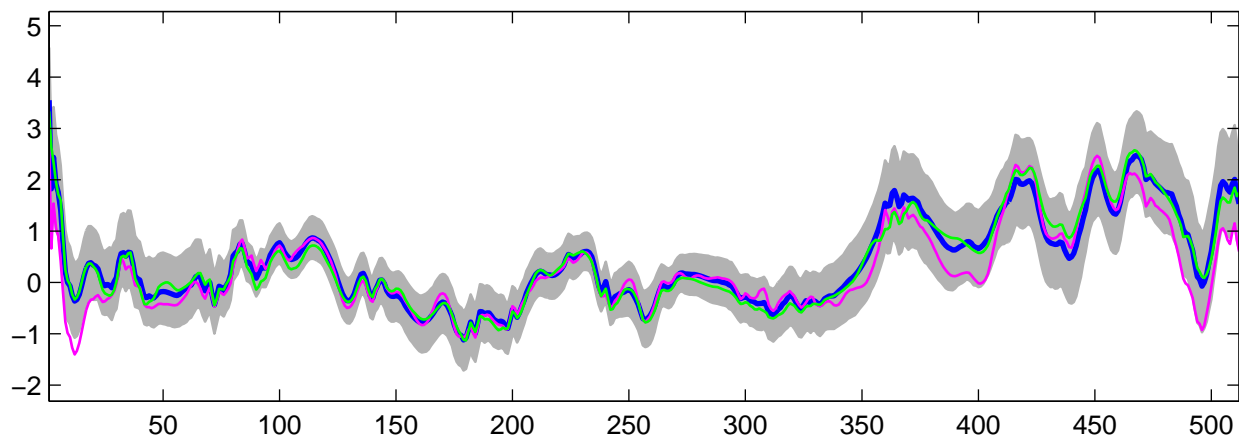
Estimated U_g(t) using R-WFMM: DE data, run 9
