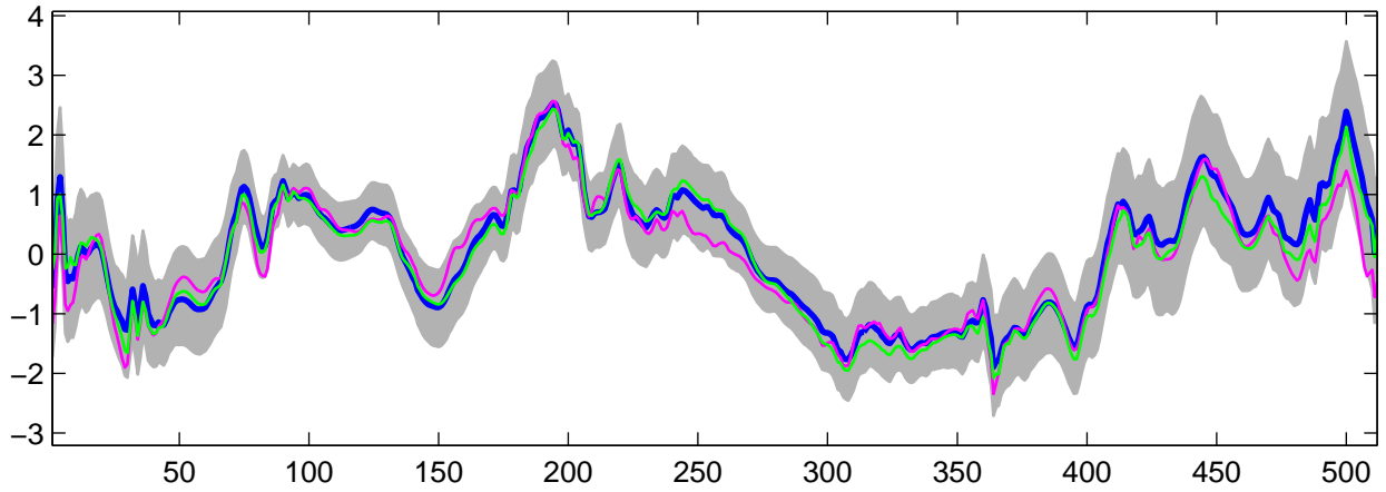
Estimated U_8(t) using G-WFMM: Normal data, run 9
