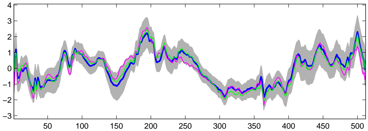
Estimated U_8(t) using R-WFMM: Normal data, run 9
