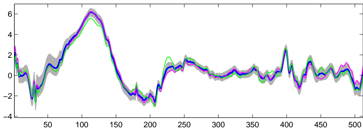
Estimated U_8(t) using R-WFMM: t_2 data, run 9
