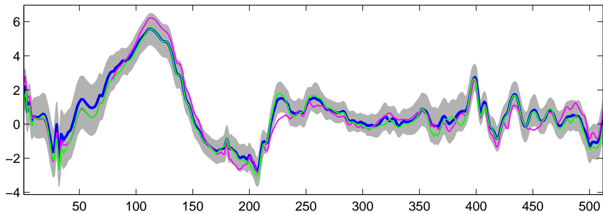
Estimated U_8(t) using G-WFMM: t_2 data, run 9
