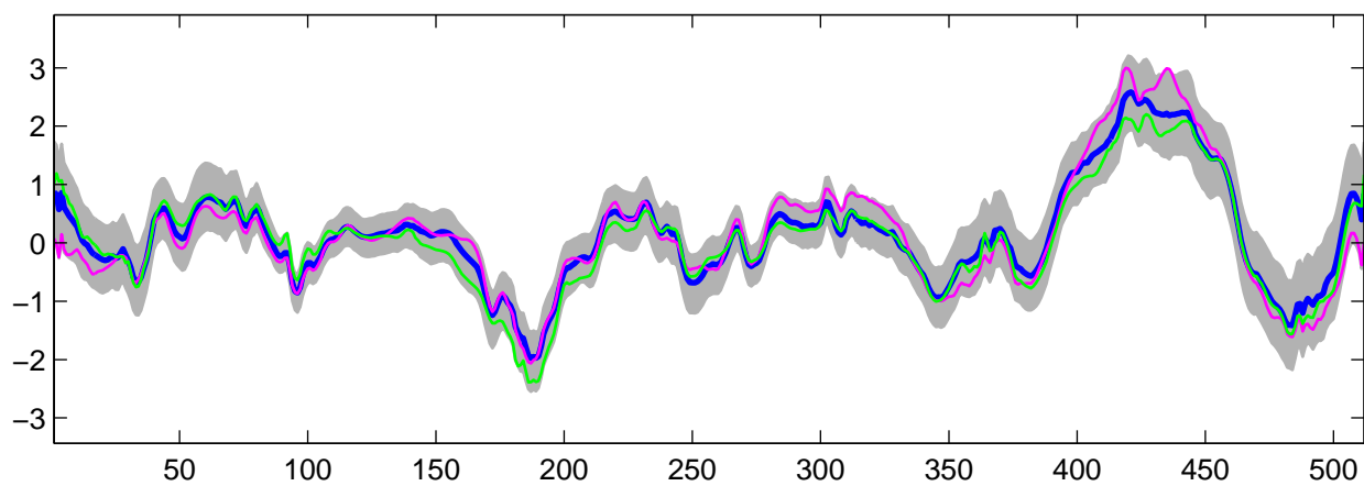
Estimated U_8(t) using R-WFMM: t_3 data, run 9
