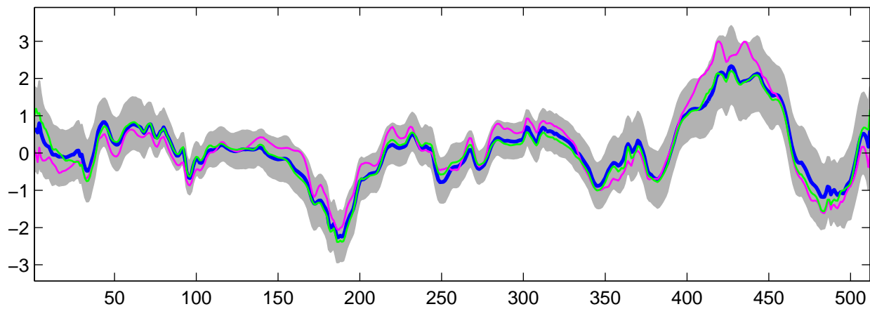
Estimated U_8(t) using G-WFMM: t_3 data, run 9
