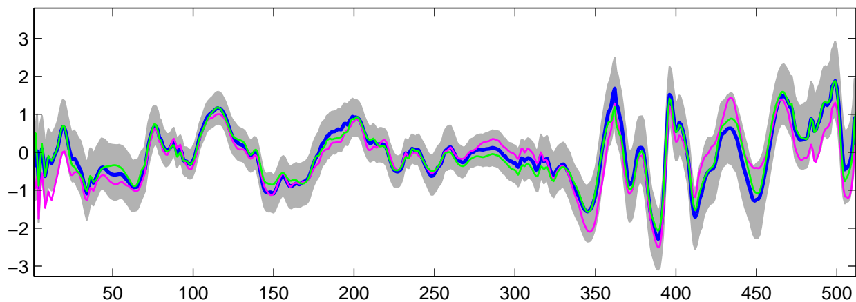
Estimated U_{\theta}(t) using R-WFMM: DE data, run 9
