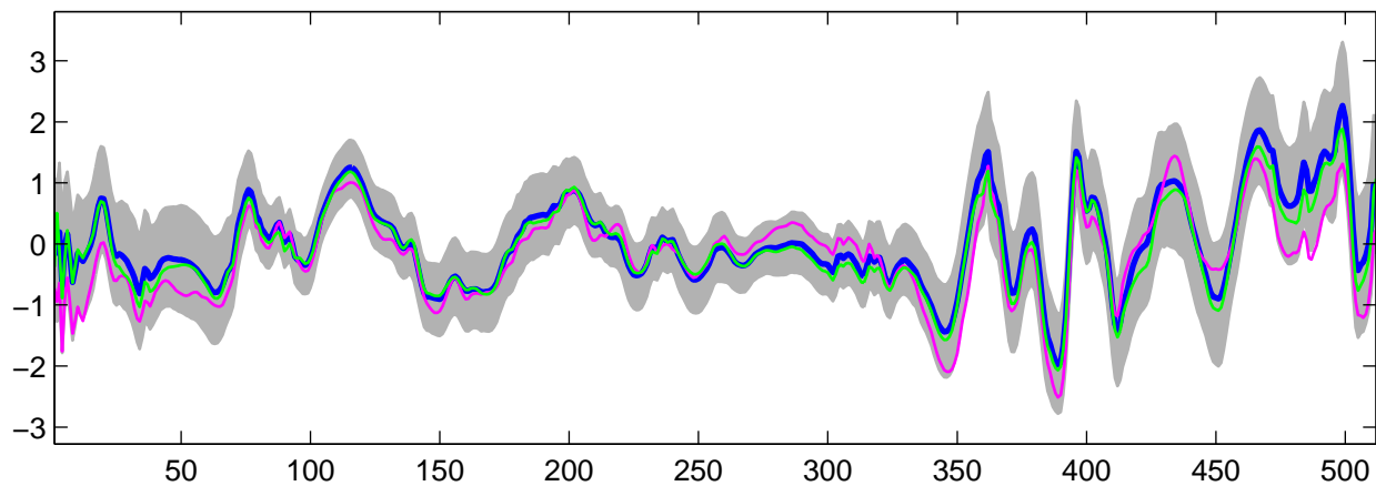
Estimated U_{\theta}(t) using G-WFMM: DE data, run 9
