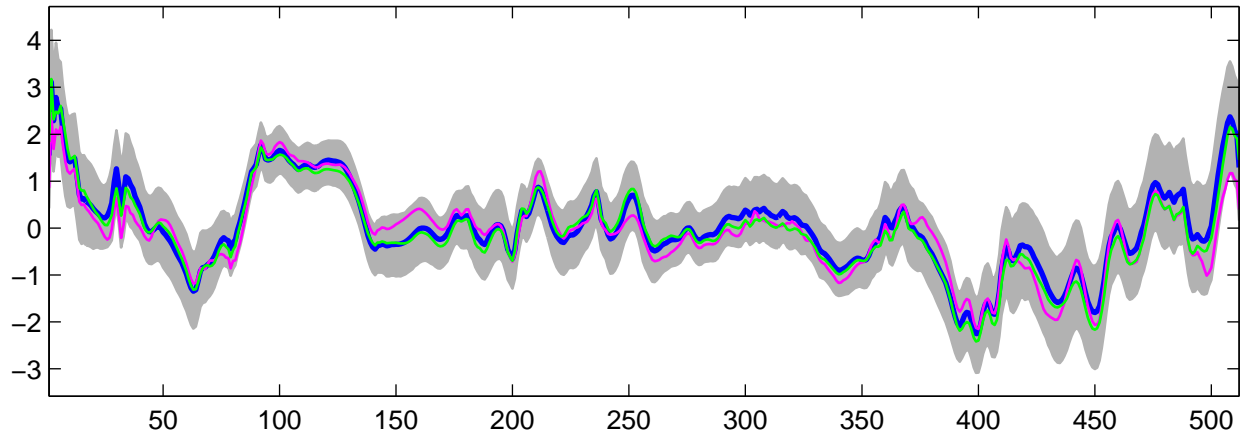
Estimated U_{\theta}(t) using G-WFMM: Normal data, run 9
