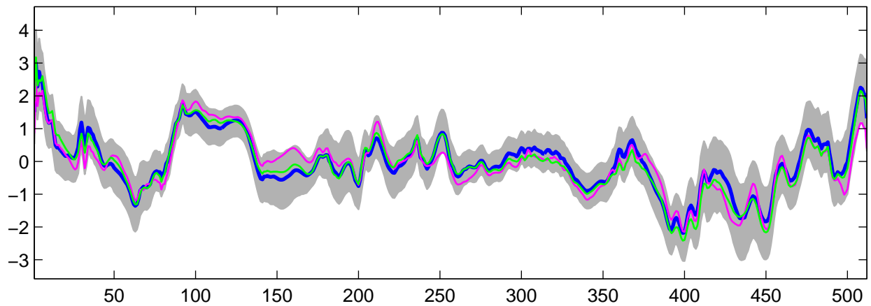
Estimated U_{\theta}(t) using R-WFMM: Normal data, run 9
