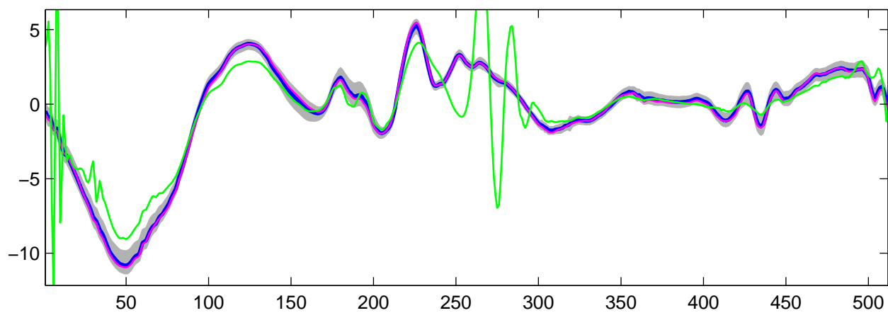
Estimated U_{\theta}(t) using R-WFMM: t_1 data, run 9
