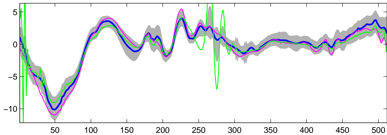
Estimated U_{\theta}(t) using G-WFMM: t_1 data, run 9
