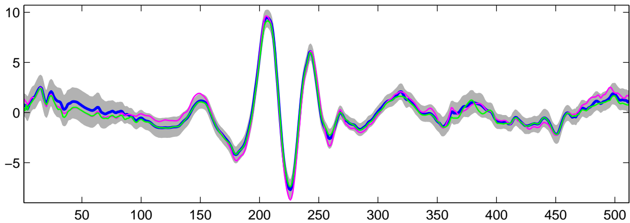
Estimated U_9(t) using G-WFMM: t_2 data, run 9
