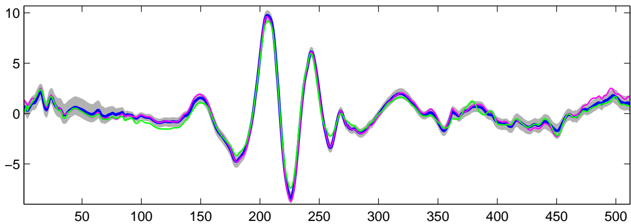
Estimated U_9(t) using R-WFMM: t_2 data, run 9
