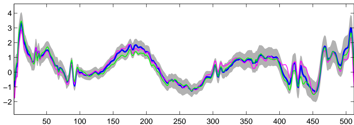
Estimated U_9(t) using R-WFMM: t_3 data, run 9
