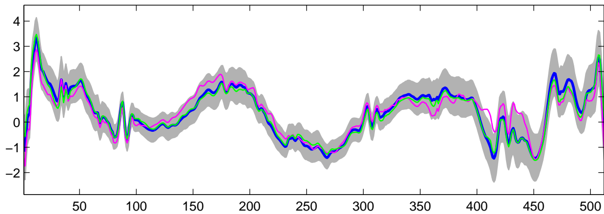
Estimated U_9(t) using G-WFMM: t_3 data, run 9
